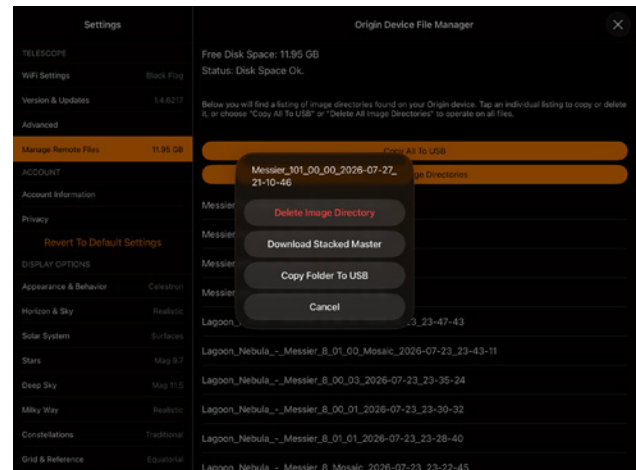
FIG I8: Download the Final Stacked Master for each tile to a USB thumbdrive from Menu>Settings>Manage Remote Files. Tap the folder for the tile, then select Copy Folder to USB. If you have turned on Save Raw Images, then the raw images files will be downloaded too.
