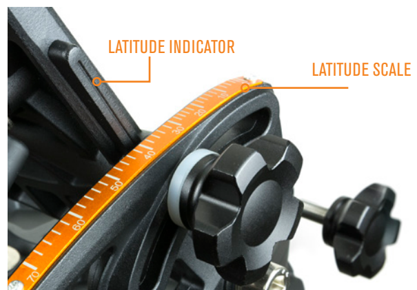
FIG D2: Turn the latitude adjustment knob on the wedge until the latitude indicator lines up with your current location's latitude on the scale.
