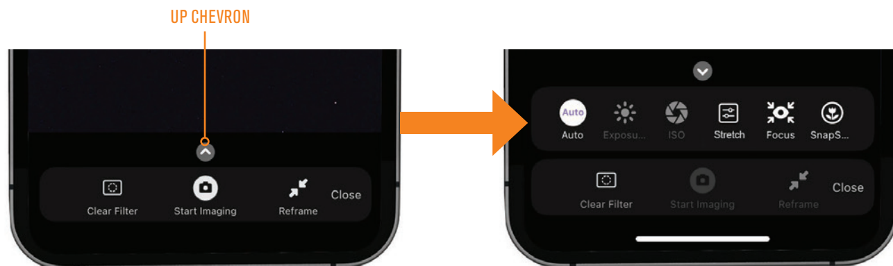
Fig. 11: Access the manual camera settings from the Camera View by pressing the up chevron.
