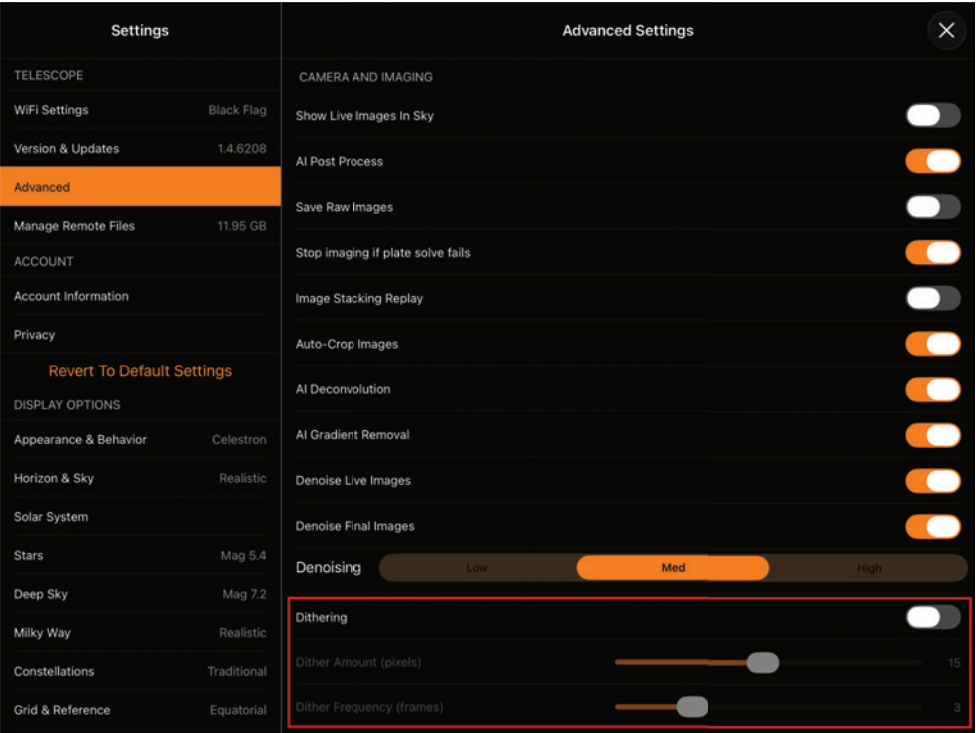
FIG H1: Origin's Dithering controls can be found under Menu>Settings>Advanced.
