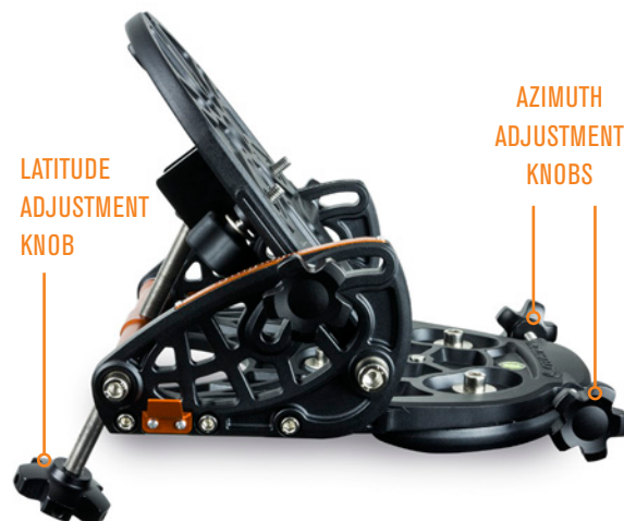
FIG D4: Make adjustments to the wedge using the azimuth and latitude adjustment knobs.
