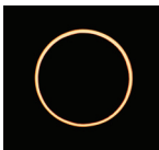
ECLIPSE ANULAR
