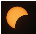
ECLIPSE PARCIAL
