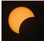
PARTIAL ECLIPSE
